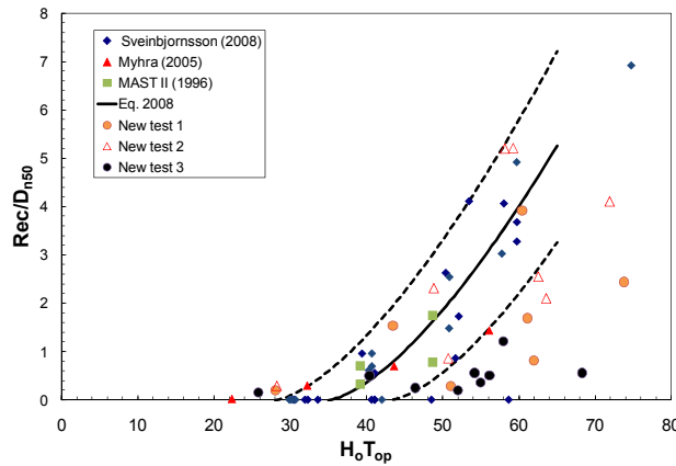
Figure 11. Average recession versus H_oT_{op} and data of Sigurdarson et al. (2008).
